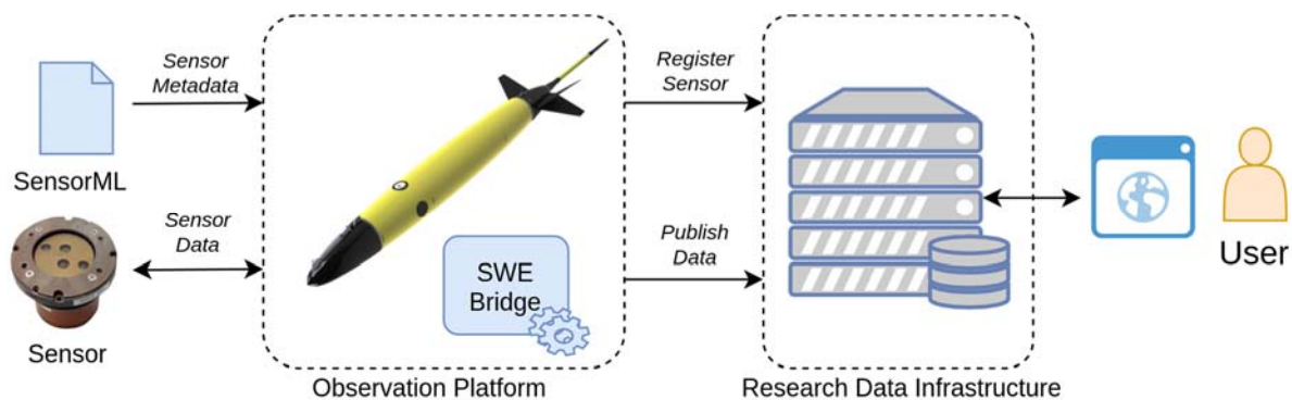
Figure 1: Automated Integration of a sensor based on SensorML metadata file into Research Data Infrastructure
