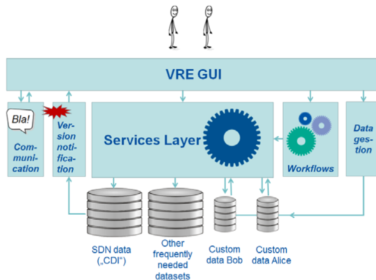
Figure 1: Architecture of the Virtual Research Environment
